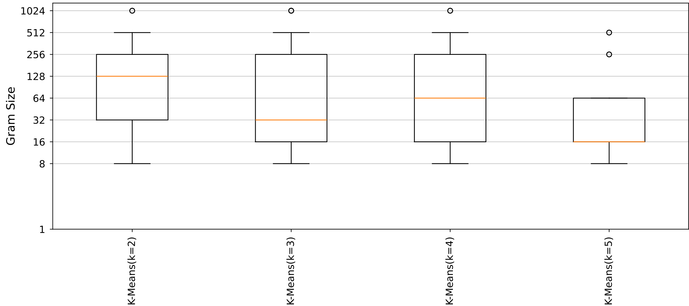
YARA Rules Gram Size Distribution (Cluster42_Size5 dataset)
